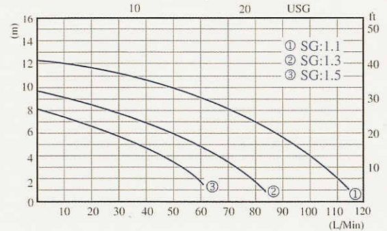
NH-200PS-Z 60Hz Nominal speed 3,300 r.p.m
