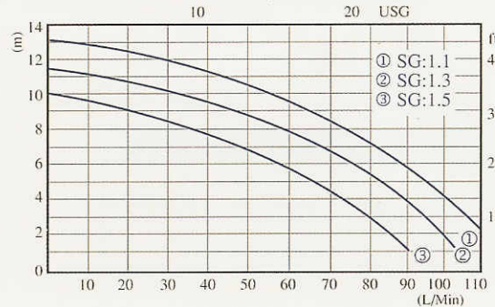
NH-250PS 50Hz Nominal speed 2,700 r.p.m
