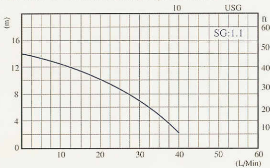
NH-200PS-Z 50Hz Nominal speed 2,500 r.p.m
